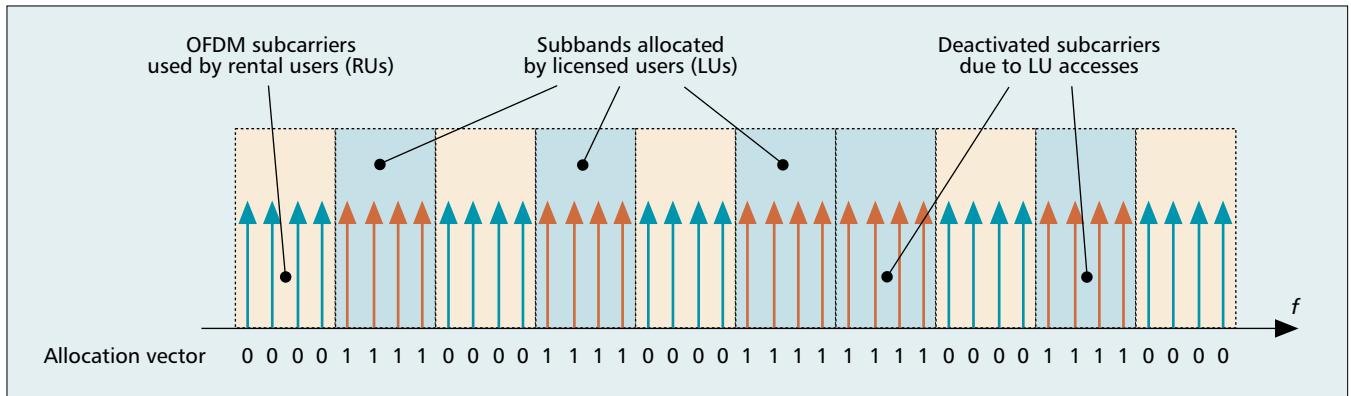
FIGURE 3. A schematic example of an OFDM-based spectrum pool.
